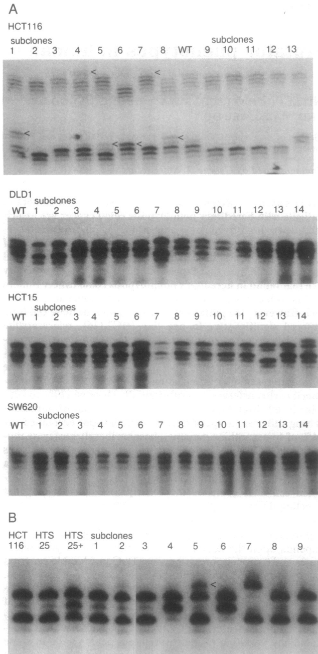
FIG. 2. Microsatellite-length variability in subclones of colorectal carcinoma cell lines. Instability was assayed at D11S527 (A) and IID (B) loci by amplification of the locus followed by fractionation of the products on a denaturing polyacrylamide gel. The gel was blotted onto Hybond-N + (Amersham) and probed with one of the primers that was labeled using terminal transferase. In A, subclones derived from each of the indicated cell lines were analyzed. In B, one of the subclones of HCT116 (designated HTS25) was resubcloned to reduce the frequency of preexisting mutants. The lane marked HTS25+ contains alleles amplified from DNA isolated from the HTS25 subclone after a longer period (~20 more generations) in culture. The mutant allele accumulates with prolonged culture, consistent with the high rate of mutation at this locus. Each lane represents an independent subclone [WT, parental (wild type) cell line]. Distinctive bands are evident in subclones of all cell lines except SW620. Marked bands (<) indicate specific alleles present in subclones that also contain both wild-type alleles. Presumably, this pattern emerges when a mutation occurs at the microsatellite locus within the first few rounds of cell division after subcloning. These events were used to calculate a mutation rate for microsatellite mutations in HCT116 cells (Table 2).
