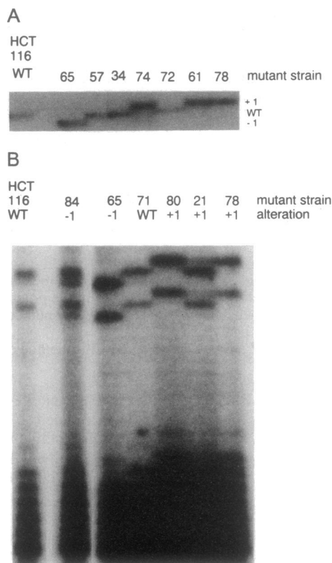
FIG. 3. Frame-shift hotspot in exon 3 of the HPRT locus in mutants isolated from HCT116. (A) Exon 3-coding sequences were amplified from DNA purified from the indicated mutant strains and fractionated on 6% denaturing polyacrylamide gels. The gel was blotted onto nitrocellulose and probed with one of the primers that was labeled using terminal transferase; this allowed rapid visualization of mutant strains with +1 or -1 frame-shifts. To determine whether the alterations of one of the fragments resulted from frame-shifts within the run of guanine residues in exon 3, the fragments were sequenced. (B) Products of reactions containing ddGTP fractionated on a 6% denaturing polyacrylamide gel. Loss (-1) or gain (+1) of guanine residues in the guanine run can be found in several of these mutant strains. In two of these mutants (strains 21 and 84), the alterations are complex, as a wild-type (WT) band and a mutant band with either a +1 or -1 frame-shift can be seen; these may result from a duplication of exon 3 occurring concurrently with the frame-shift. Frame-shifts at this site were found in 24% of HPRT mutant strains obtained from HCT116.
